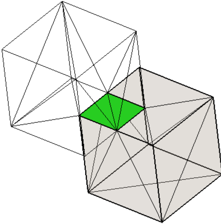
Fig. 7 in green the triangulation of the two faces (identical) that “were” the shared face
